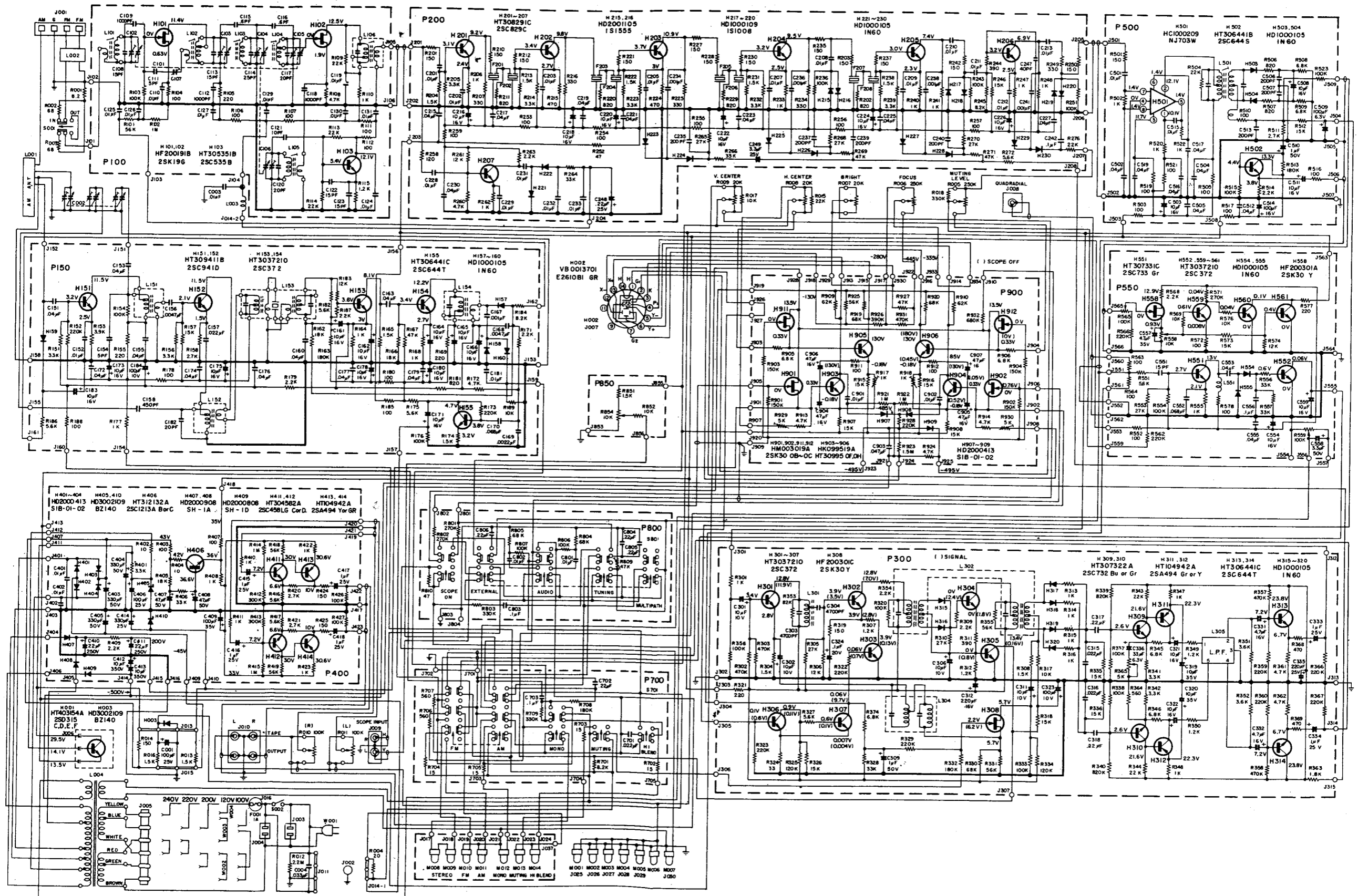
Figure 19. Schematic Diagram
